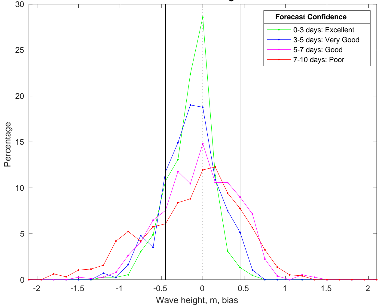
NDBC 42020 vs CMEMS Waves Bias Histogram: 22-Mar-2025
