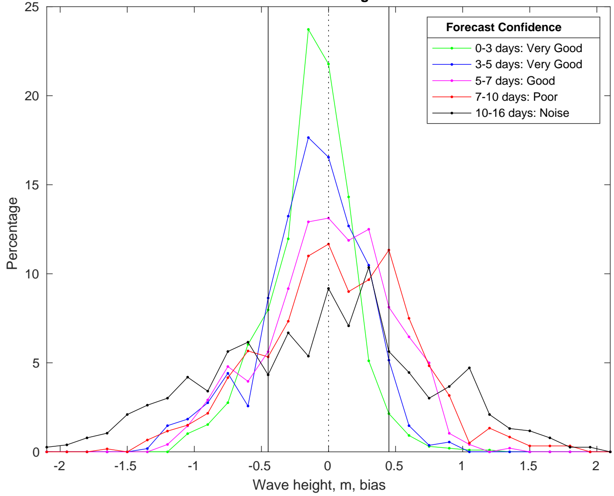
NDBC 42020 vs GFS Waves Bias Histogram: 22-Mar-2025
