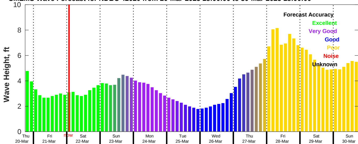
CMEMS Wave Forecast for NDBC 42020 from 20-Mar-2025 18:00:00 to 30-Mar-2025 18:00:00
