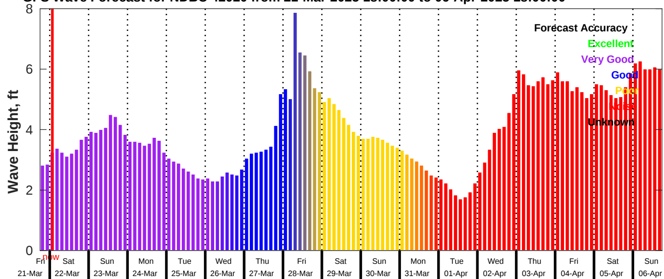
GFS Wave Forecast for NDBC 42020 from 21-Mar-2025 18:00:00 to 06-Apr-2025 18:00:00
