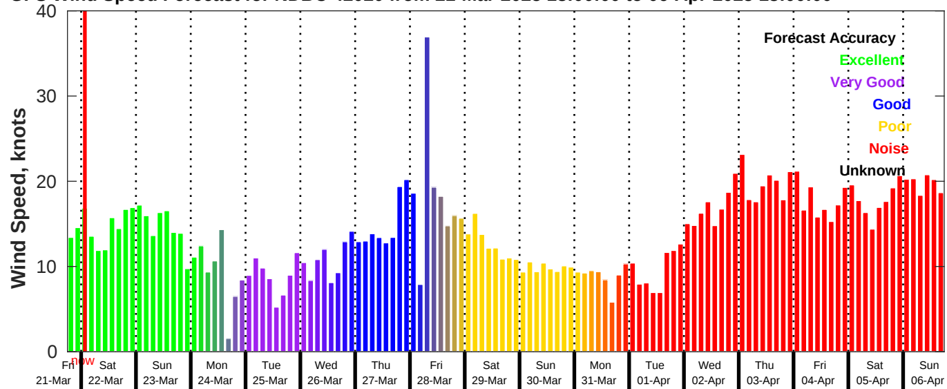
GFS Wind Speed Forecast for NDBC 42020 from 21-Mar-2025 18:00:00 to 06-Apr-2025 18:00:00
