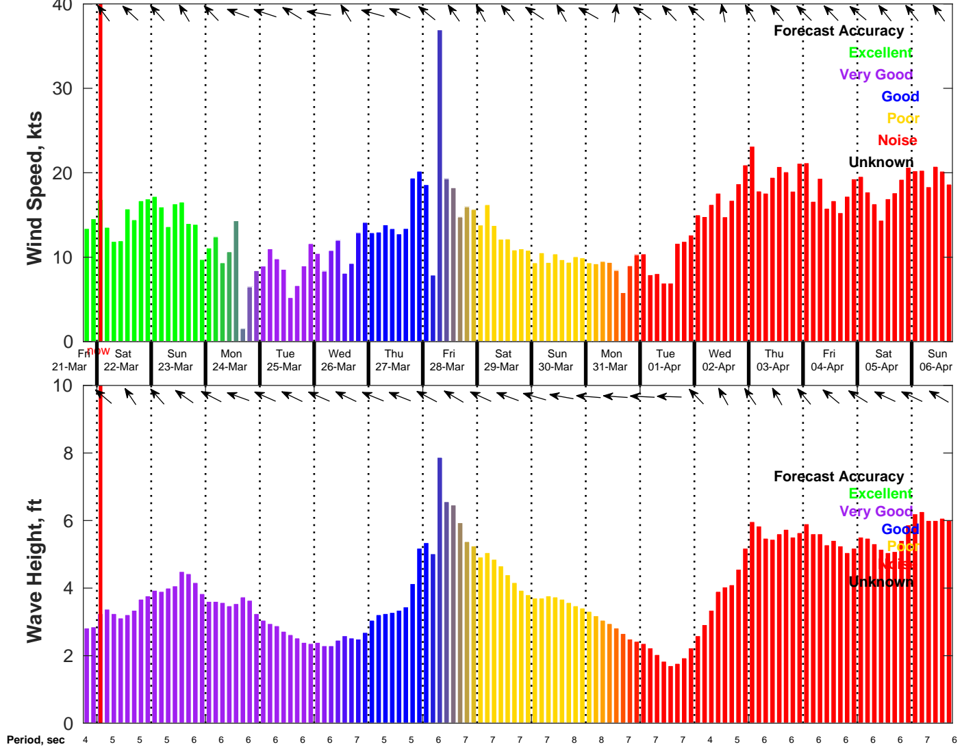
Wind & Wave Forecast for NDBC 42020 from 21-Mar-2025 18:00:00 to 06-Apr-2025 18:00:00
