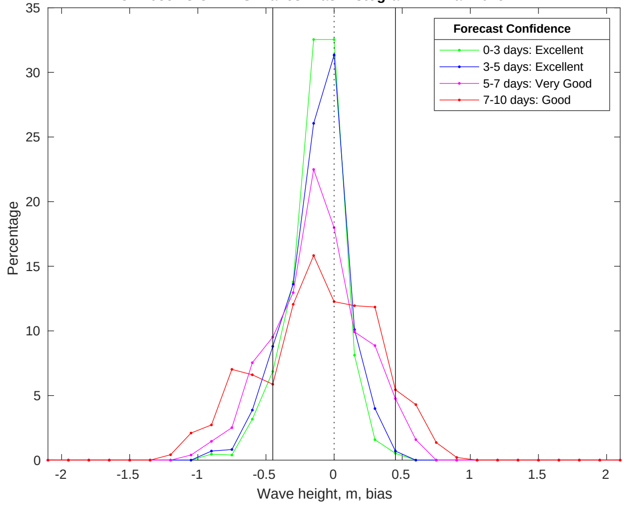
NDBC 42035 vs CMEMS Waves Bias Histogram: 22-Mar-2025
