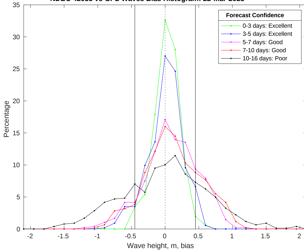
NDBC 42035 vs GFS Waves Bias Histogram: 22-Mar-2025
