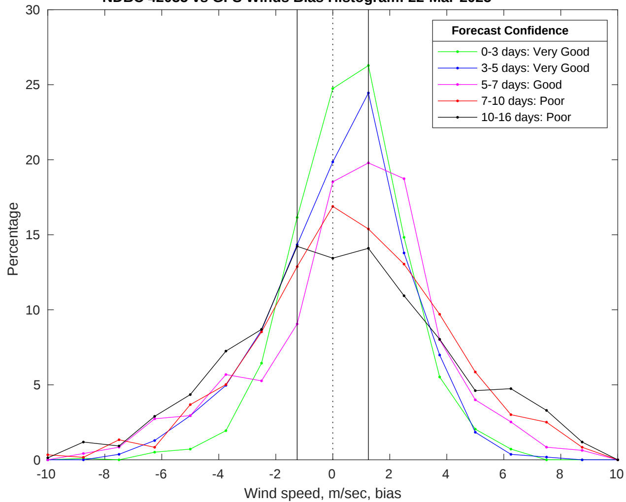
NDBC 42035 vs GFS Winds Bias Histogram: 22-Mar-2025
