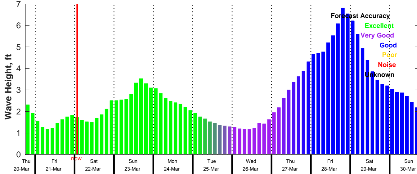
CMEMS Wave Forecast for NDBC 42035 from 20-Mar-2025 18:00:00 to 30-Mar-2025 18:00:00
