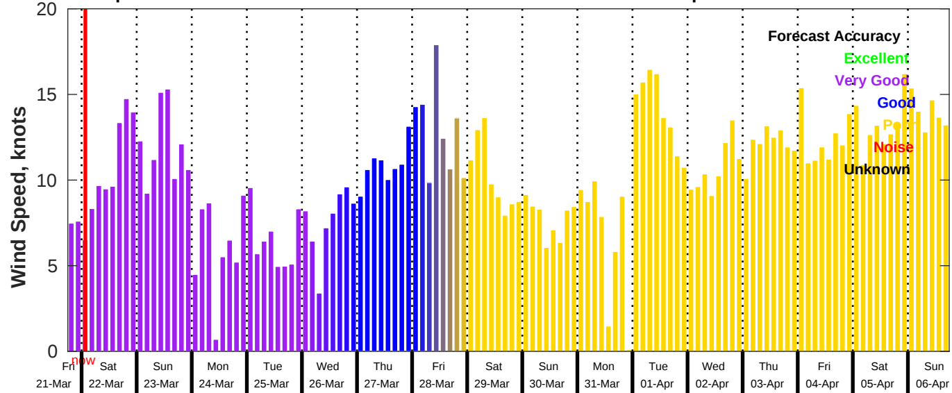
GFS Wind Speed Forecast for NDBC 42035 from 21-Mar-2025 18:00:00 to 06-Apr-2025 18:00:00
