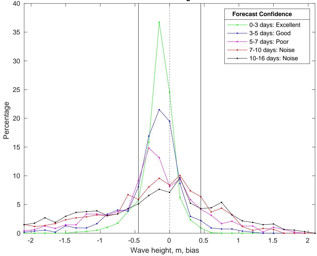
NDBC 42036 vs GFS Waves Bias Histogram: 22-Mar-2025
