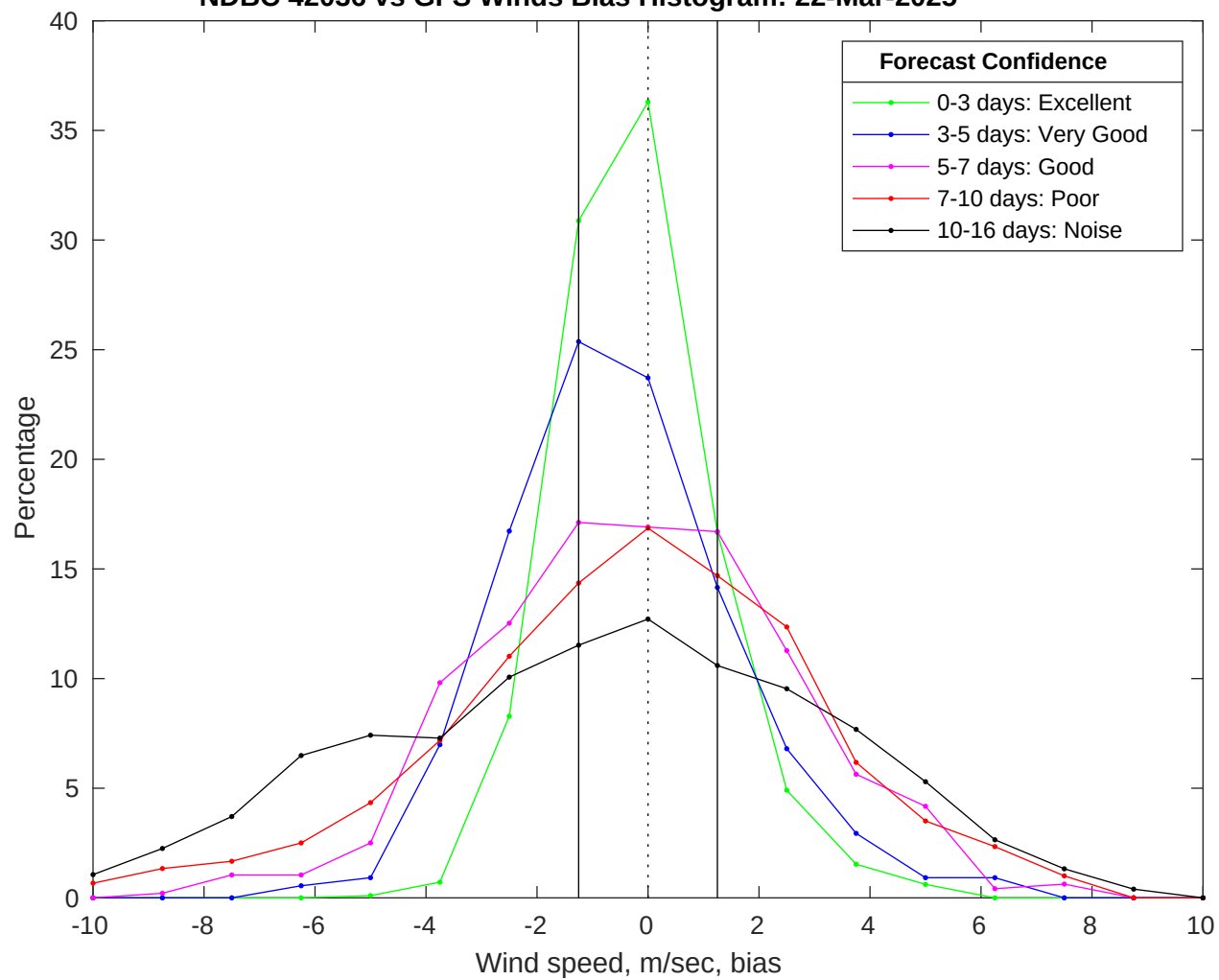
NDBC 42036 vs GFS Winds Bias Histogram: 22-Mar-2025
