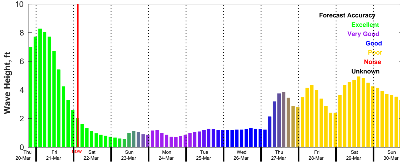
CMEMS Wave Forecast for NDBC 42036 from 20-Mar-2025 19:00:00 to 30-Mar-2025 19:00:00
