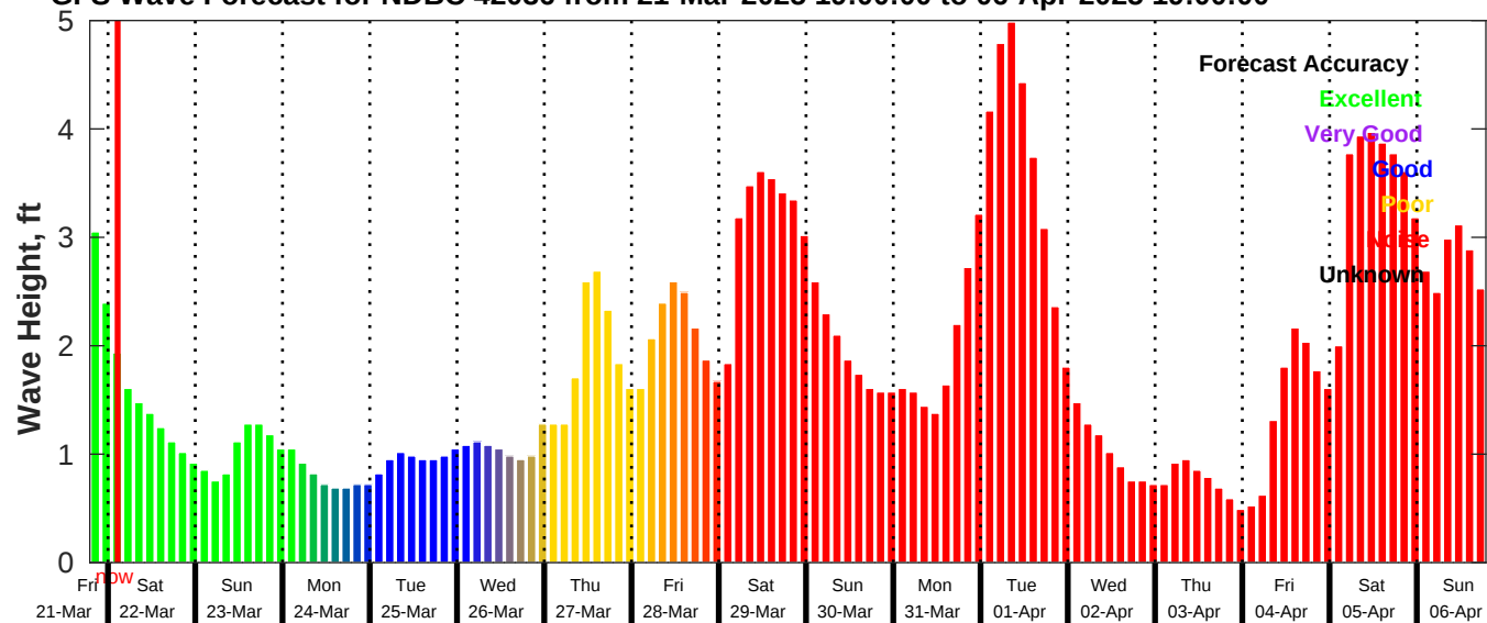
GFS Wave Forecast for NDBC 42036 from 21-Mar-2025 19:00:00 to 06-Apr-2025 19:00:00
