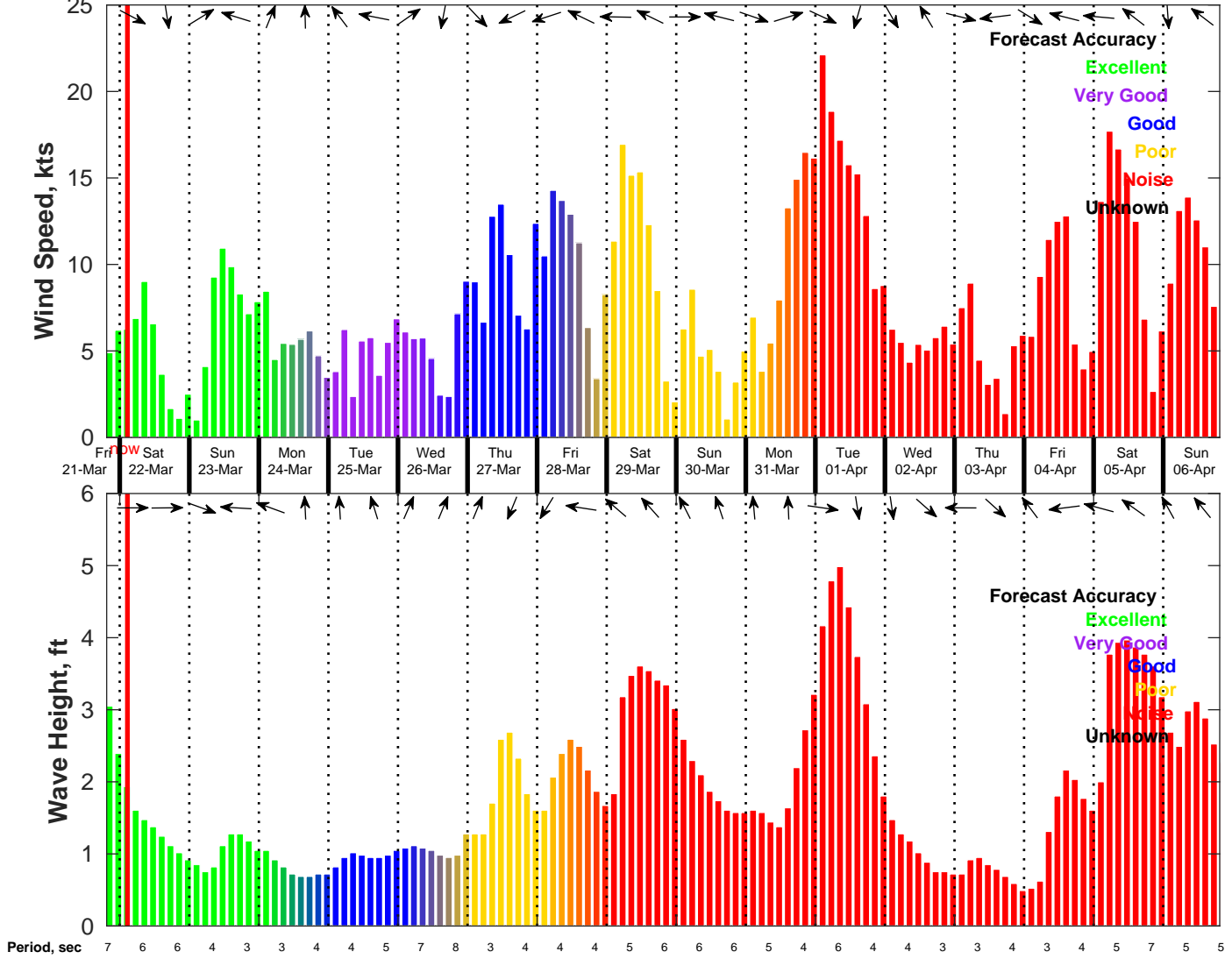
Wind & Wave Forecast for NDBC 42036 from 21-Mar-2025 19:00:00 to 06-Apr-2025 19:00:00
