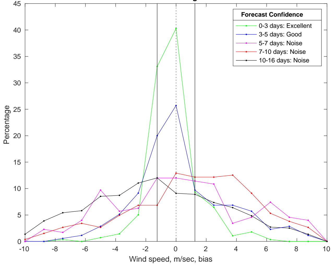
NDBC 42040 vs GFS Winds Bias Histogram: 22-Mar-2025
