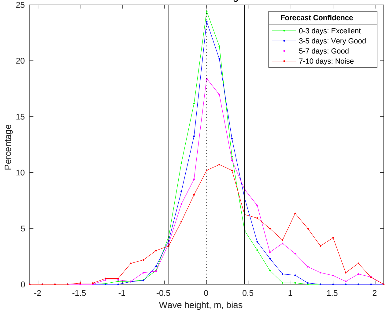
NDBC 46011 vs CMEMS Waves Bias Histogram: 22-Mar-2025
