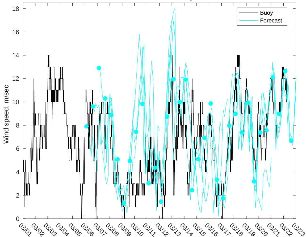
NDBC 46011 vs GFS Winds: 5 to 7 day forecast
