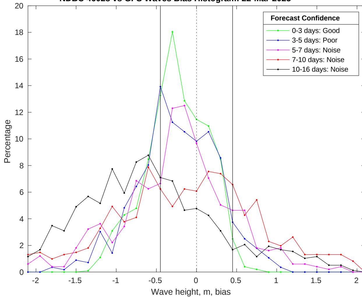
NDBC 46028 vs GFS Waves Bias Histogram: 22-Mar-2025
