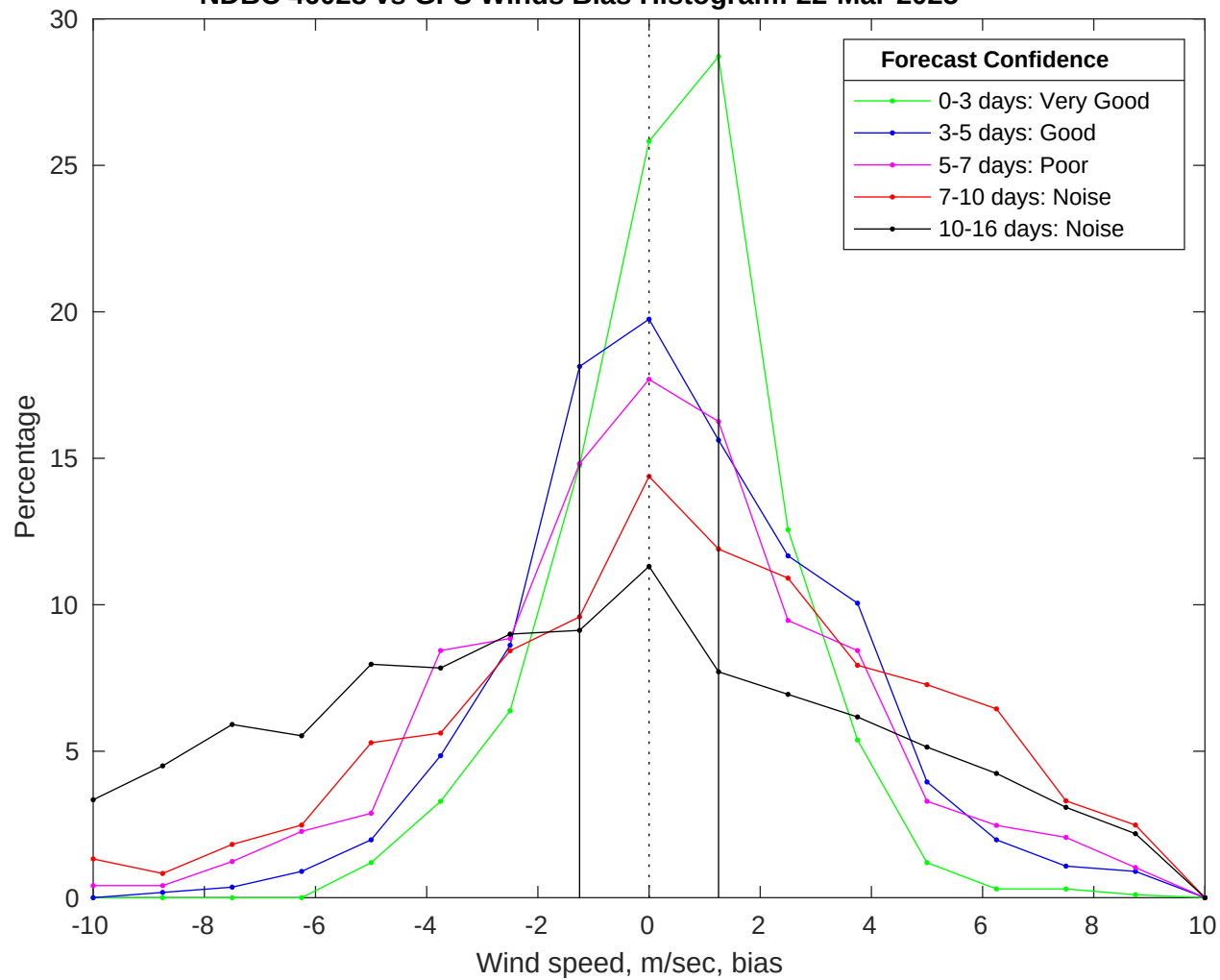
NDBC 46028 vs GFS Winds Bias Histogram: 22-Mar-2025
