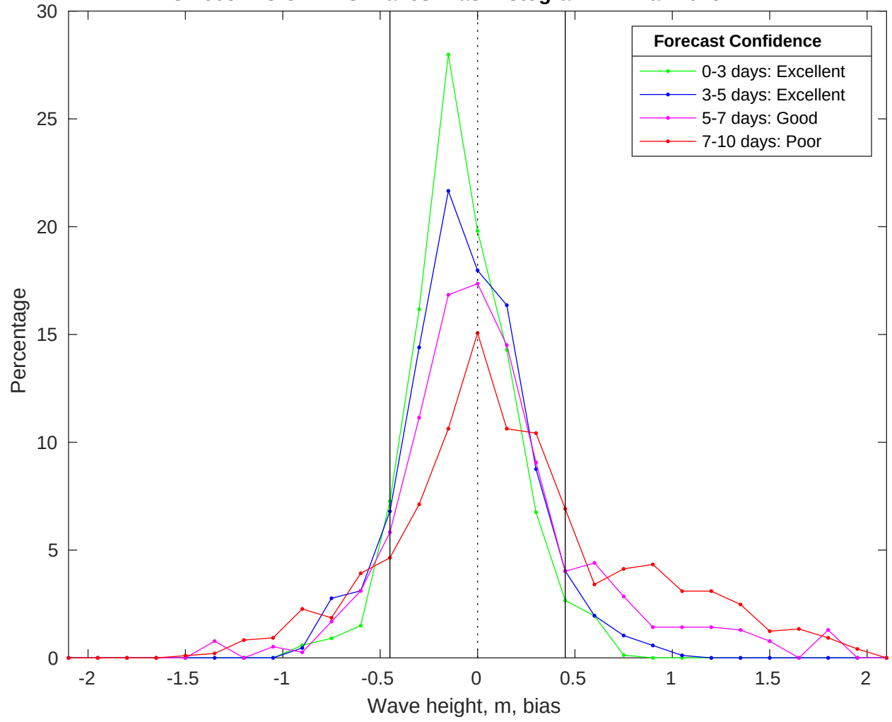
NDBC 46054 vs CMEMS Waves Bias Histogram: 22-Mar-2025
