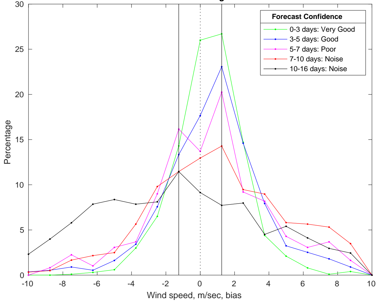
NDBC 46054 vs GFS Winds Bias Histogram: 22-Mar-2025
