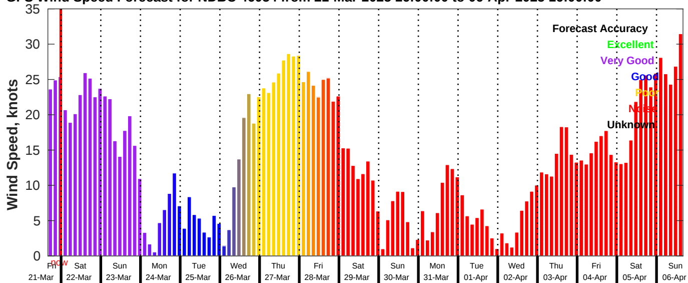
GFS Wind Speed Forecast for NDBC 46054 from 21-Mar-2025 16:00:00 to 06-Apr-2025 16:00:00
