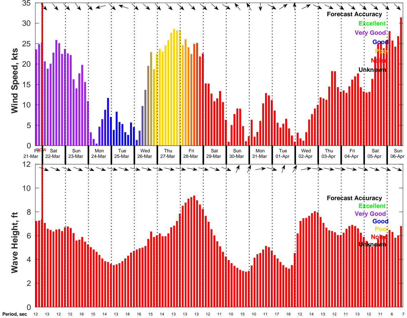
Wind & Wave Forecast for NDBC 46054 from 21-Mar-2025 16:00:00 to 06-Apr-2025 16:00:00
