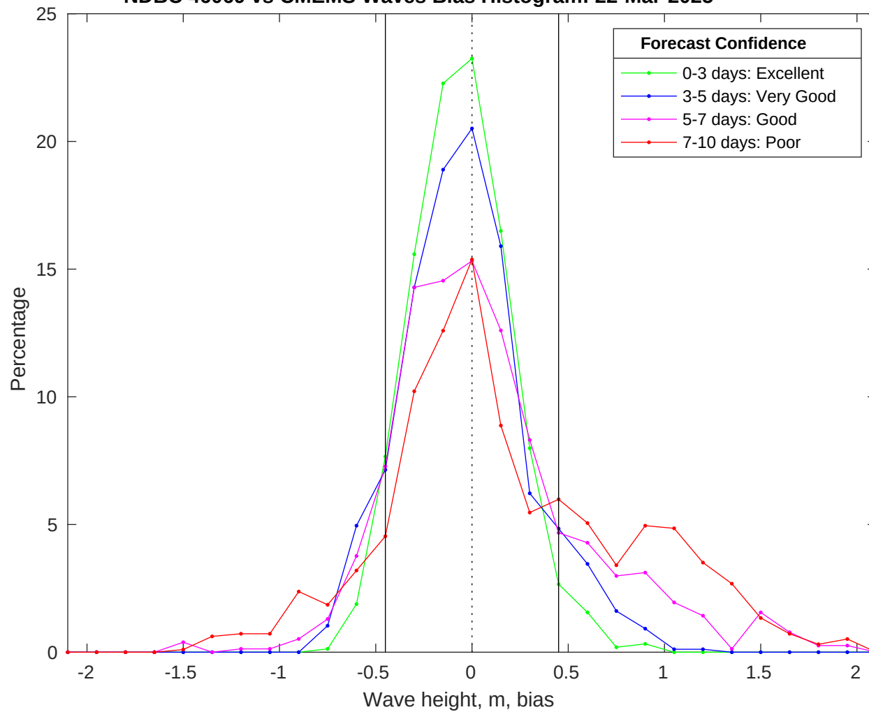
NDBC 46069 vs CMEMS Waves Bias Histogram: 22-Mar-2025
