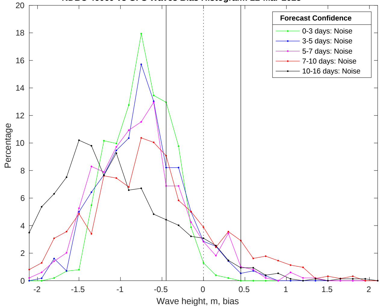
NDBC 46069 vs GFS Waves Bias Histogram: 22-Mar-2025
