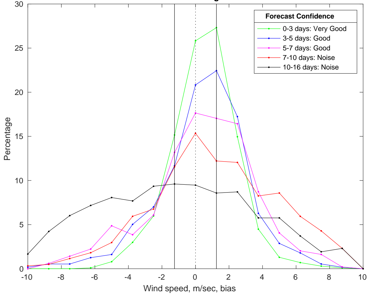
NDBC 46069 vs GFS Winds Bias Histogram: 22-Mar-2025
