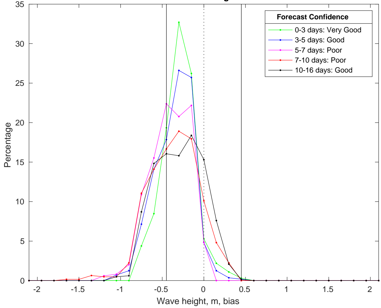
NDBC 51209 vs GFS Waves Bias Histogram: 22-Mar-2025
