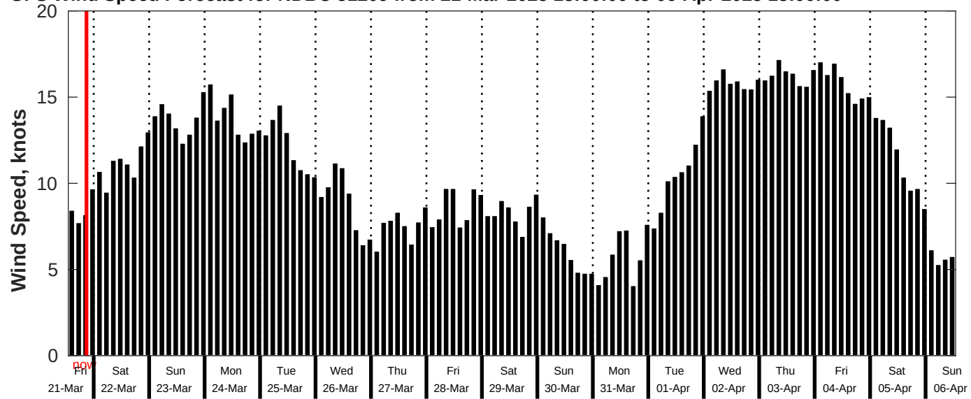
GFS Wind Speed Forecast for NDBC 51209 from 21-Mar-2025 13:00:00 to 06-Apr-2025 13:00:00
