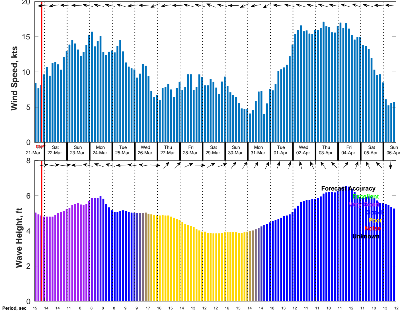
Wind & Wave Forecast for NDBC 51209 from 21-Mar-2025 13:00:00 to 06-Apr-2025 13:00:00
