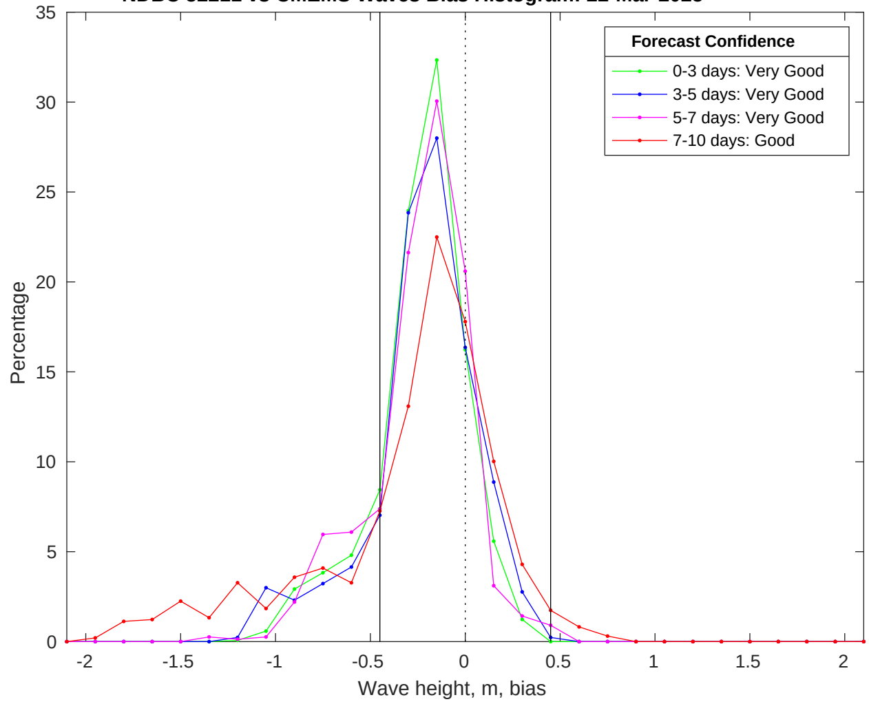
NDBC 52211 vs CMEMS Waves Bias Histogram: 22-Mar-2025
