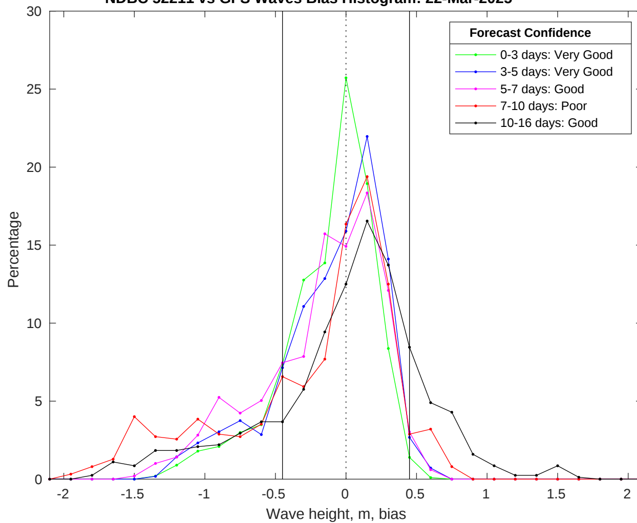
NDBC 52211 vs GFS Waves Bias Histogram: 22-Mar-2025
