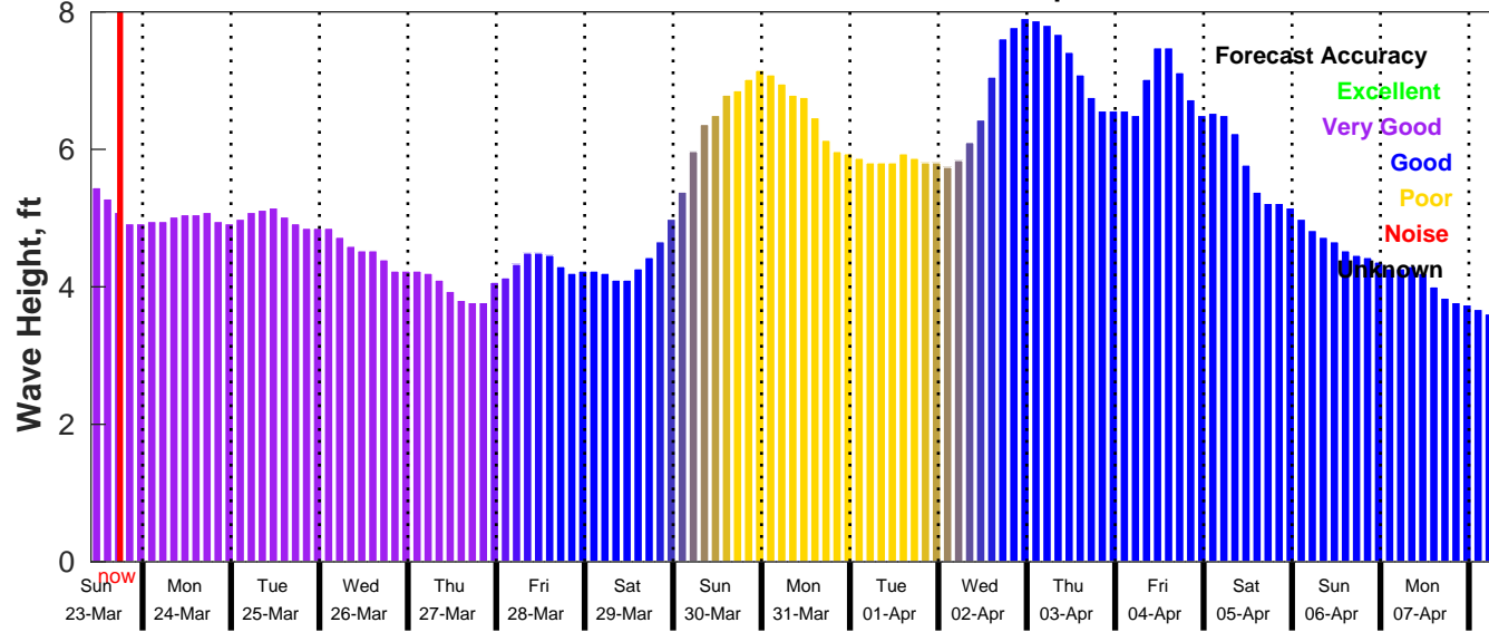
GFS Wave Forecast for NDBC 52211 from 22-Mar-2025 10:00:00 to 07-Apr-2025 10:00:00
