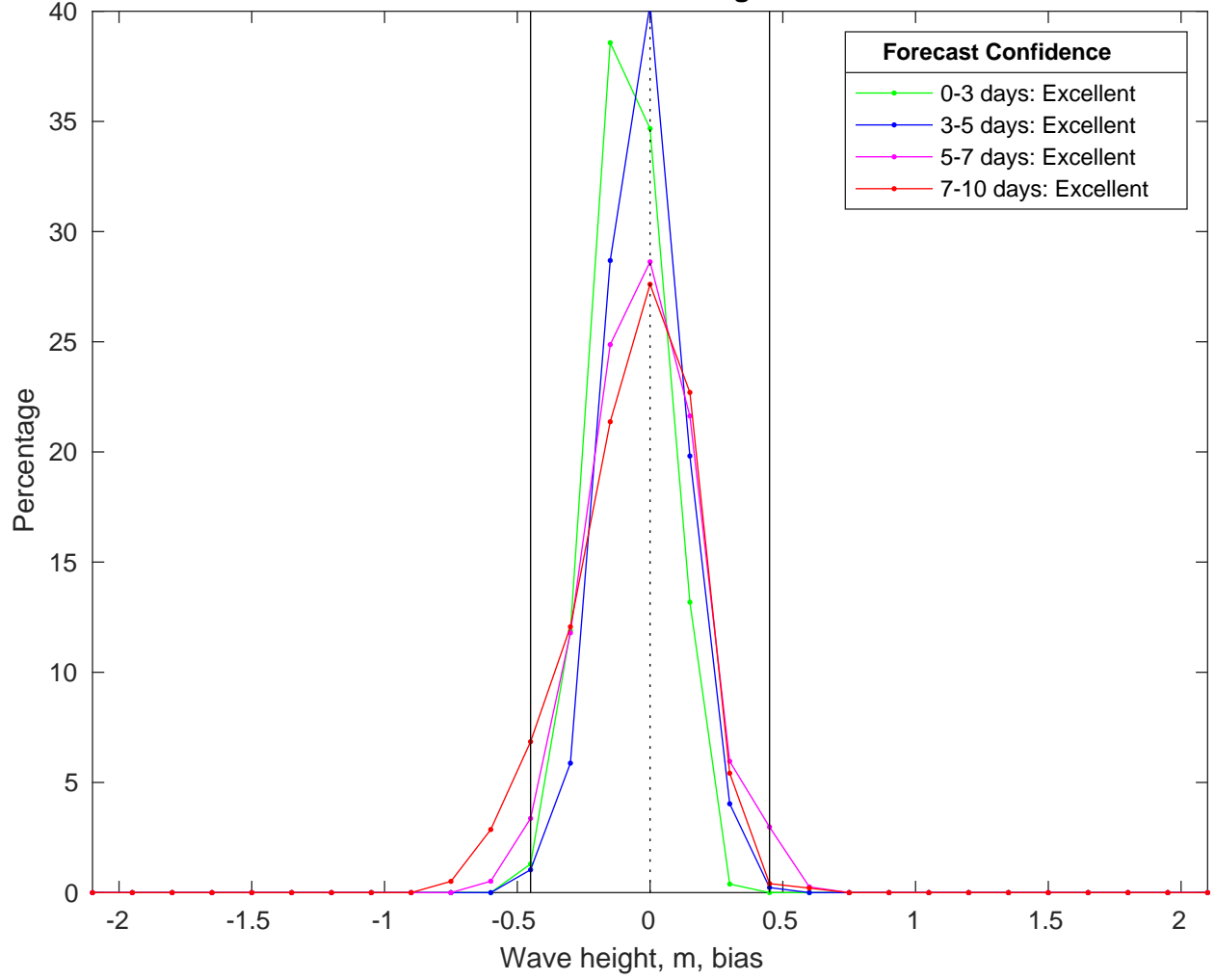
NDBC 52212 vs CMEMS Waves Bias Histogram: 22-Mar-2025
