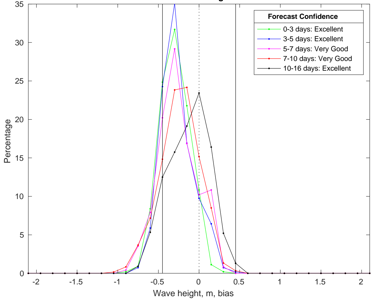
NDBC 52212 vs GFS Waves Bias Histogram: 22-Mar-2025
