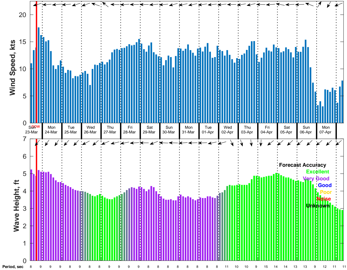
Wind & Wave Forecast for NDBC 52212 from 22-Mar-2025 09:00:00 to 07-Apr-2025 09:00:00
