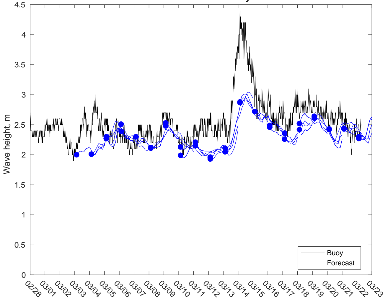
NDBC 52213 vs CMEMS Waves: 3 to 5 day forecast
