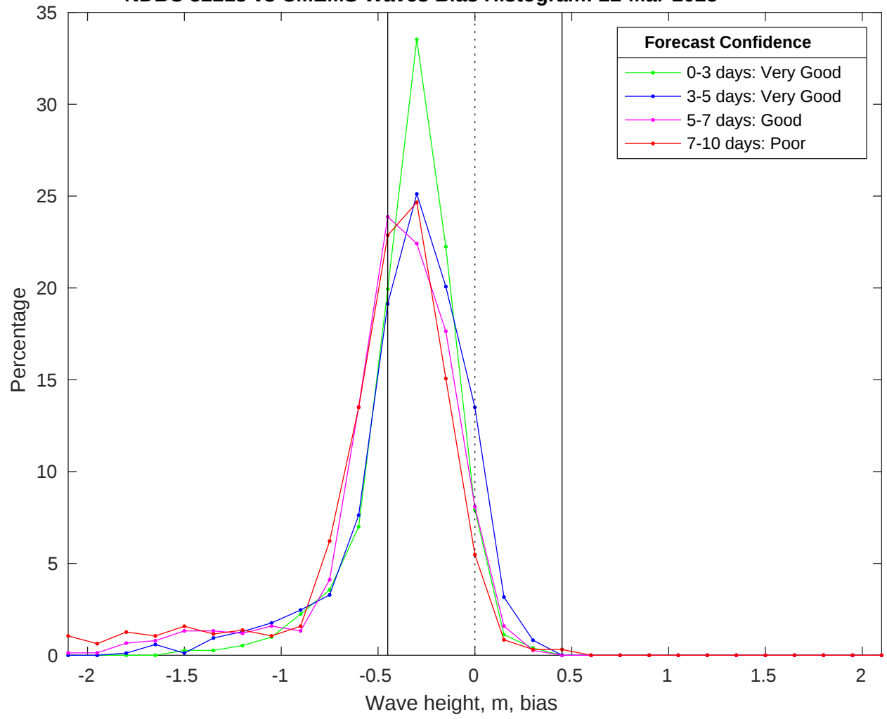
NDBC 52213 vs CMEMS Waves Bias Histogram: 22-Mar-2025
