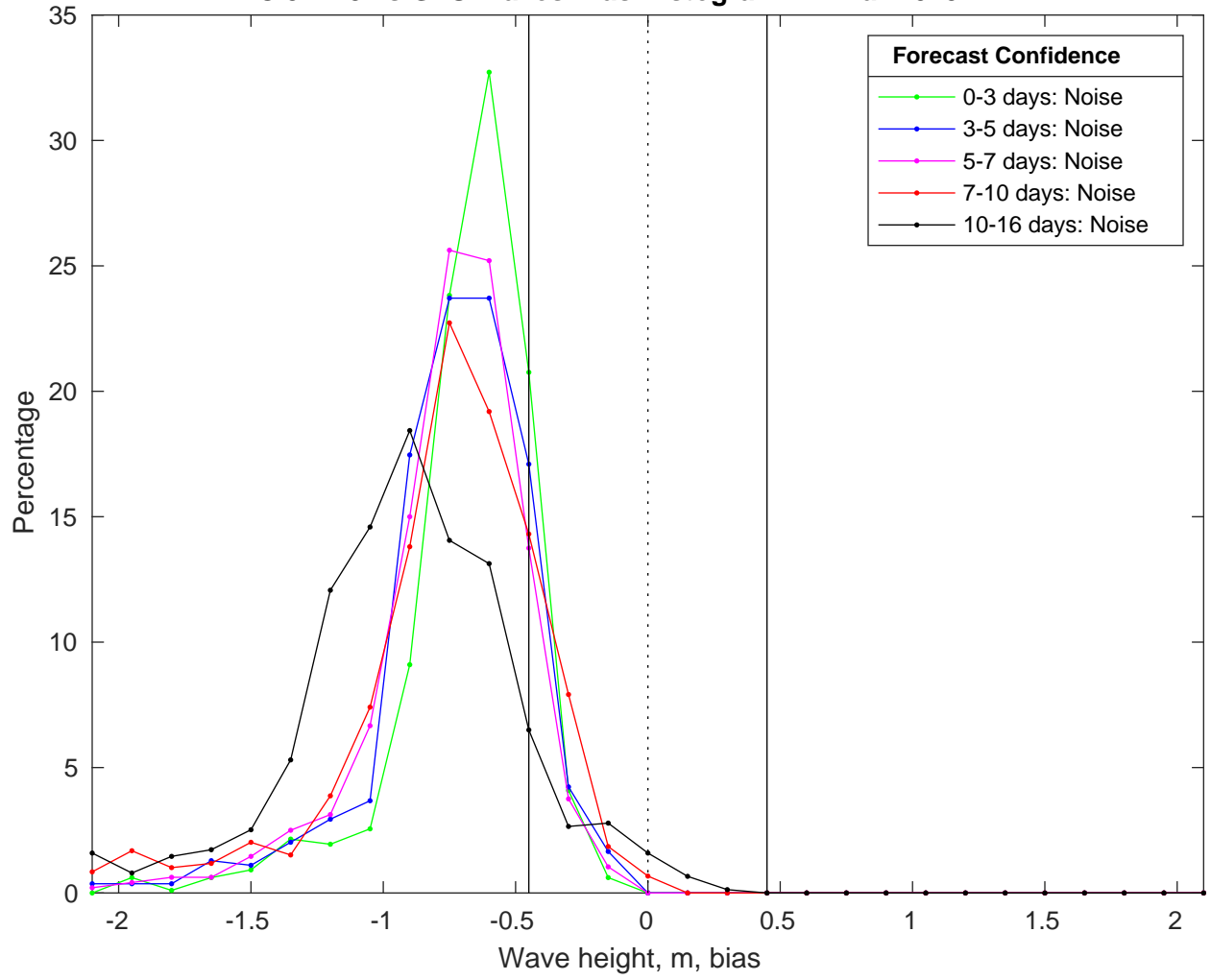
NDBC 52213 vs GFS Waves Bias Histogram: 22-Mar-2025
