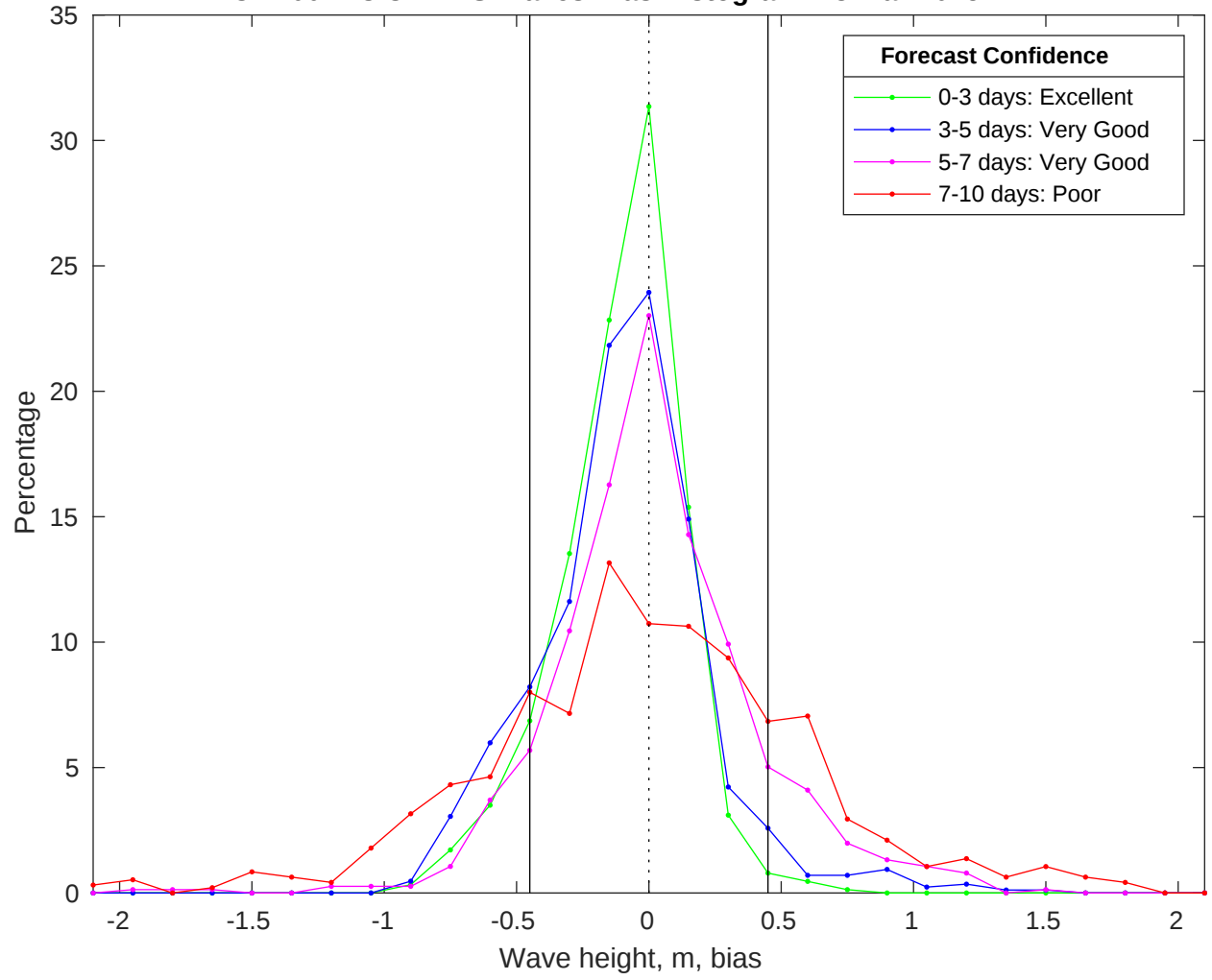
NDBC 41004 vs CMEMS Waves Bias Histogram: 23-Mar-2025
