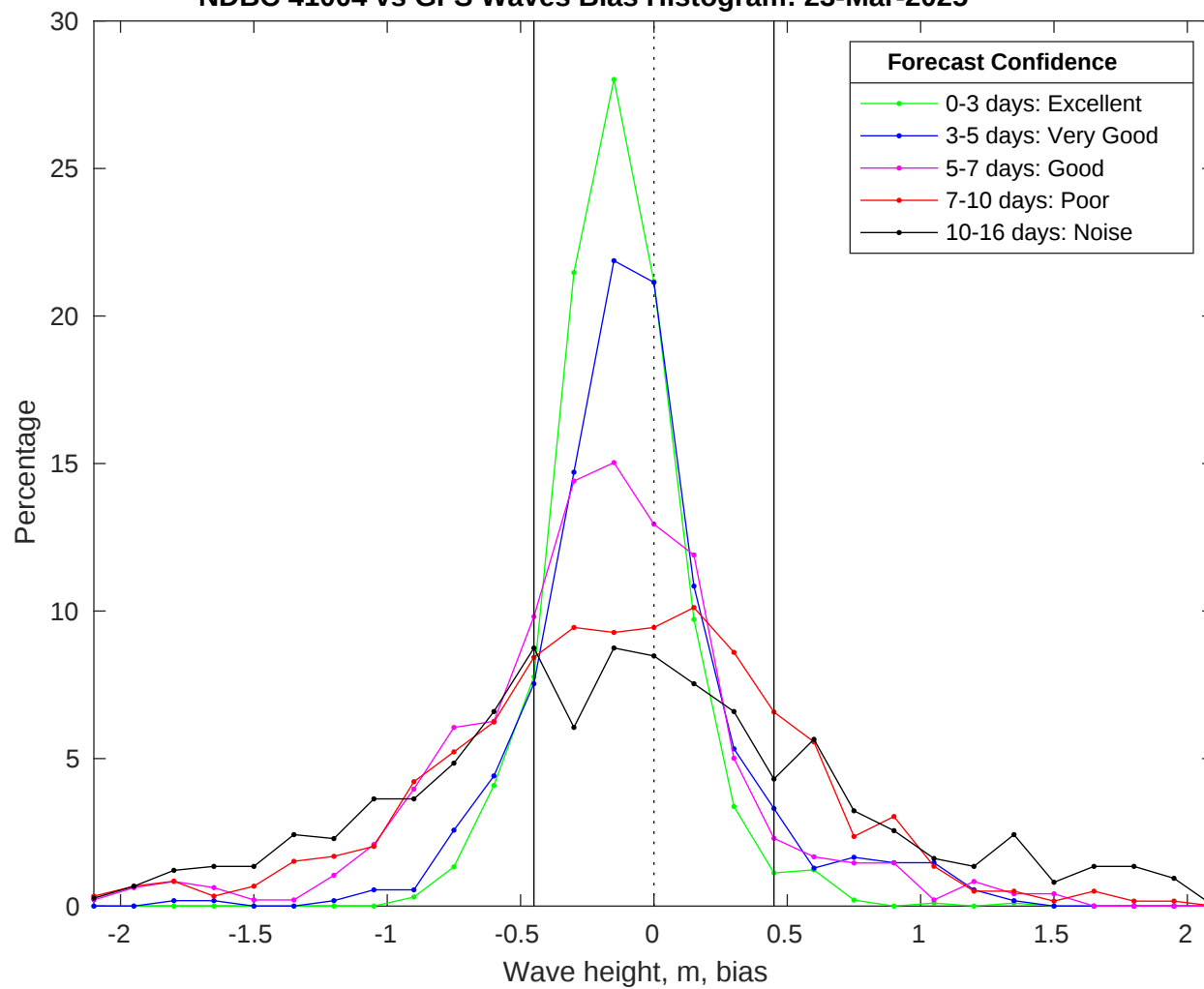
NDBC 41004 vs GFS Waves Bias Histogram: 23-Mar-2025
