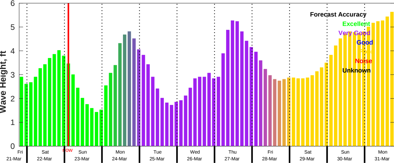
CMEMS Wave Forecast for NDBC 41004 from 21-Mar-2025 19:00:00 to 31-Mar-2025 19:00:00
