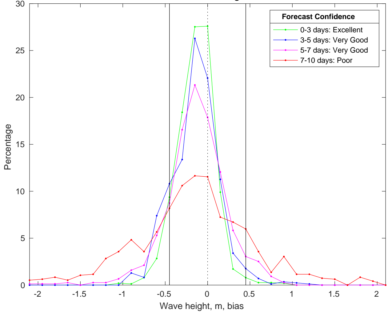
NDBC 41013 vs CMEMS Waves Bias Histogram: 23-Mar-2025
