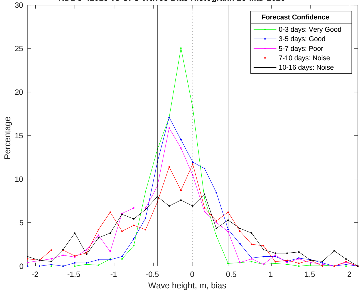
NDBC 41013 vs GFS Waves Bias Histogram: 23-Mar-2025
