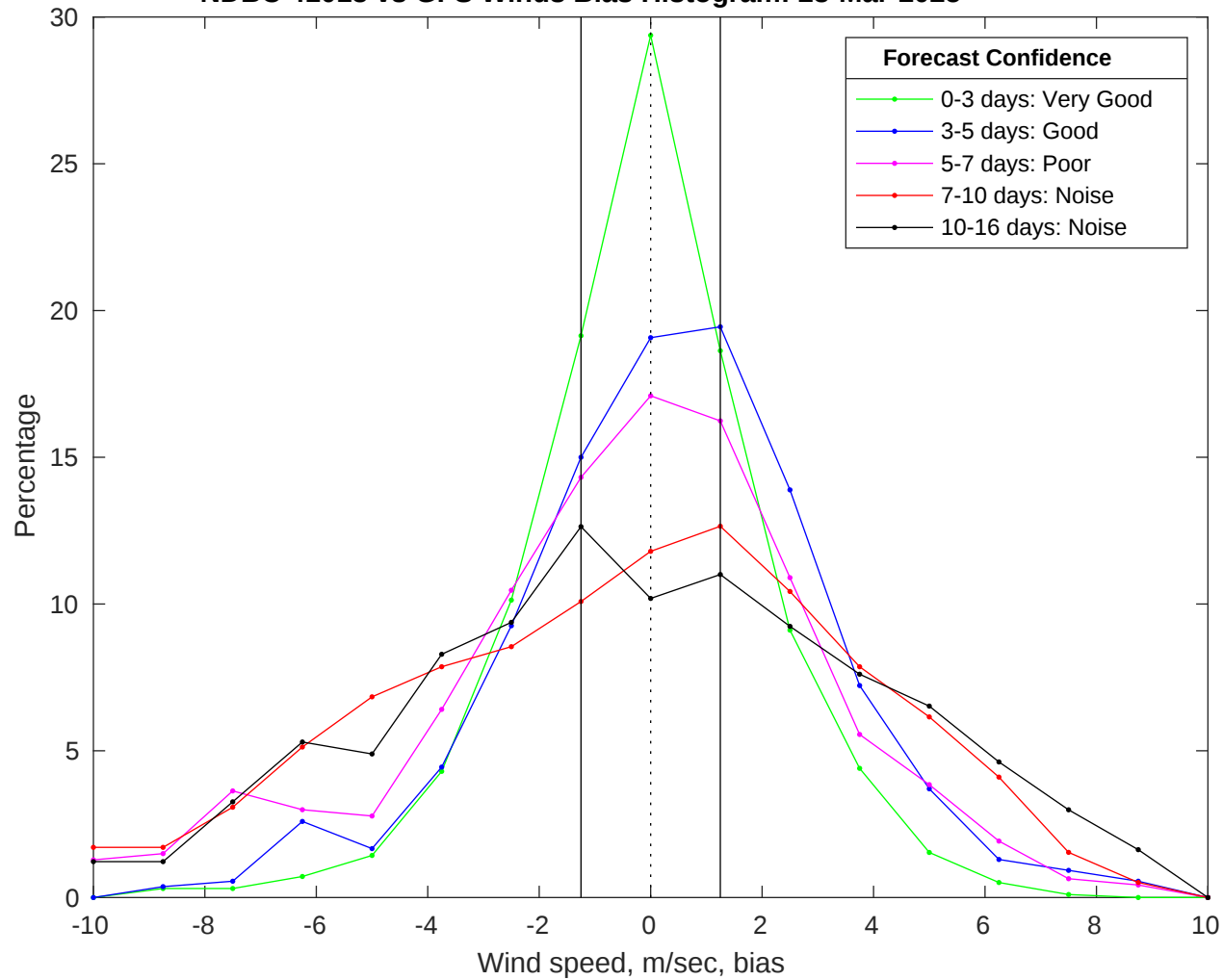
NDBC 41013 vs GFS Winds Bias Histogram: 23-Mar-2025
