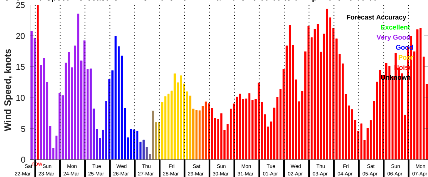
GFS Wind Speed Forecast for NDBC 41013 from 22-Mar-2025 19:00:00 to 07-Apr-2025 19:00:00
