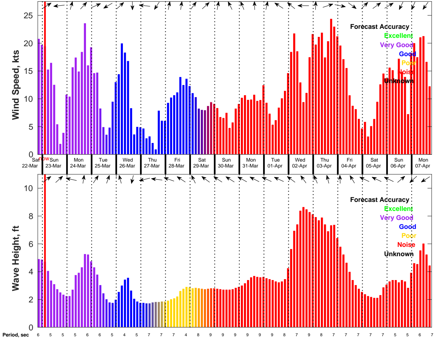
Wind & Wave Forecast for NDBC 41013 from 22-Mar-2025 19:00:00 to 07-Apr-2025 19:00:00
