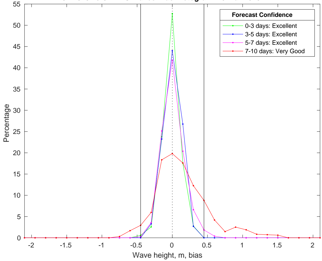
NDBC 41040 vs CMEMS Waves Bias Histogram: 23-Mar-2025
