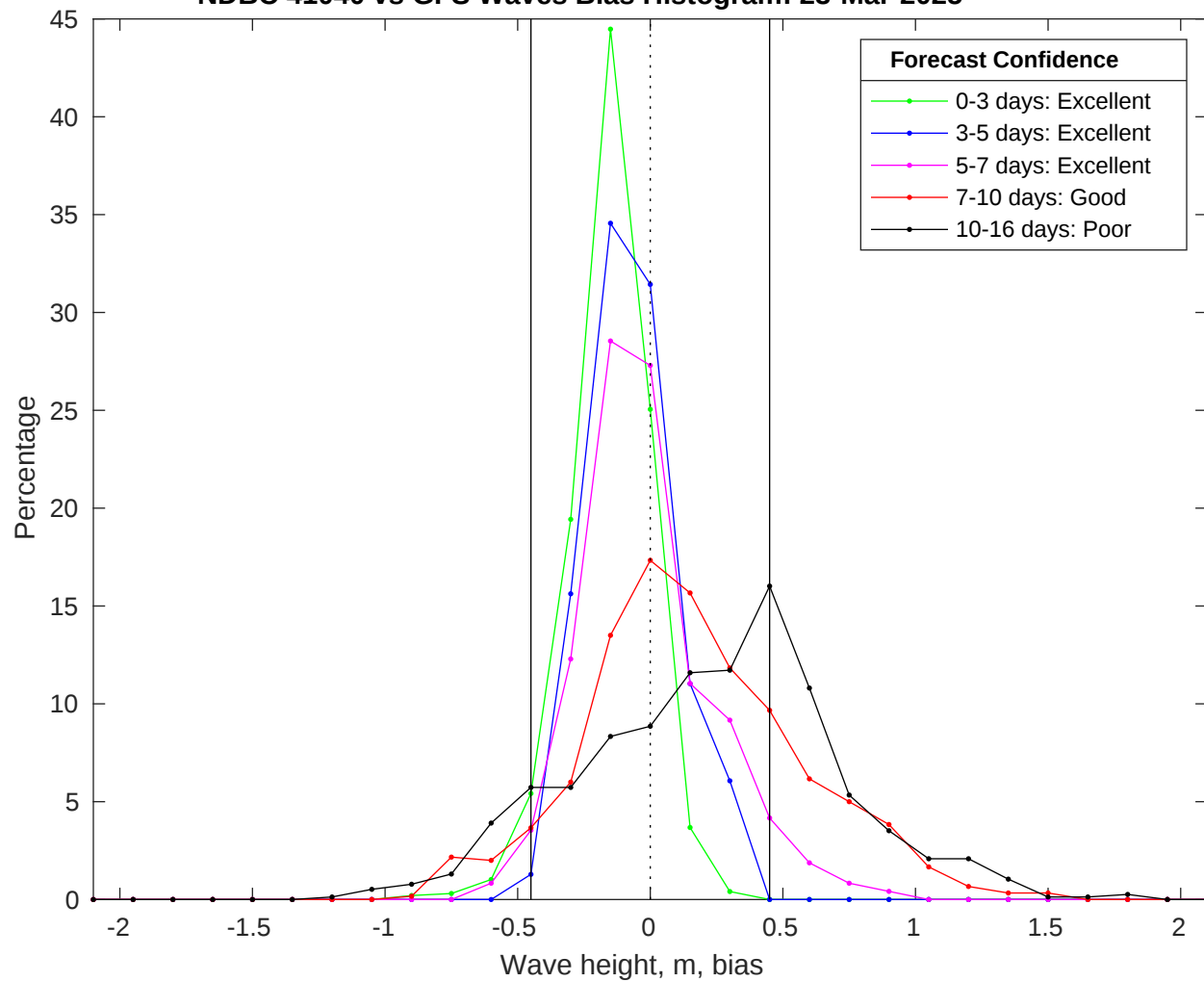
NDBC 41040 vs GFS Waves Bias Histogram: 23-Mar-2025
